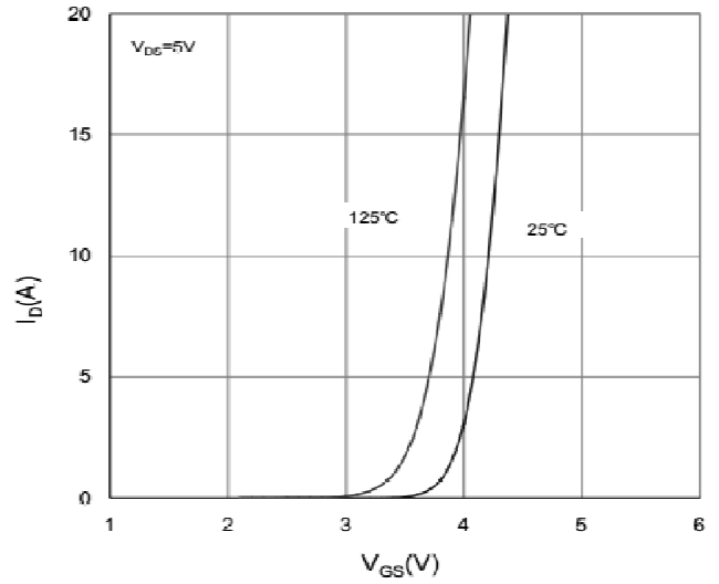
Transfer Characteristic
