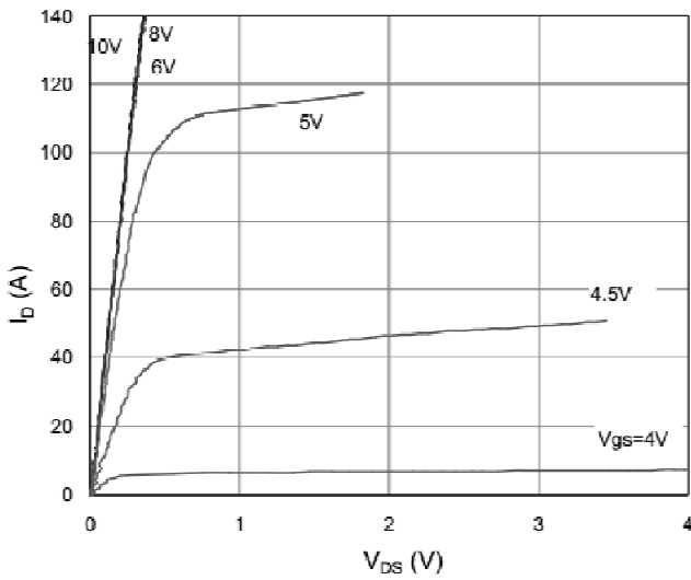
Output Characteristic
